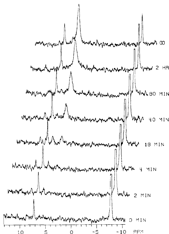
Figure 2. 2 H NMR vs. time of the reaction of DMn(CO) 5 with 1a , 0 °C in toluene (C 6 D 6 added as reference).
